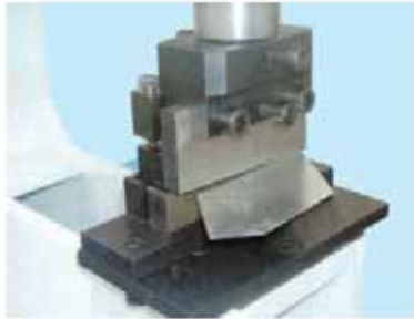
Shear Kit Max capacity: 16ga. Mild steel
