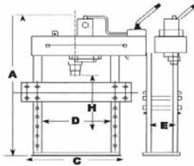
Technical Drawing
